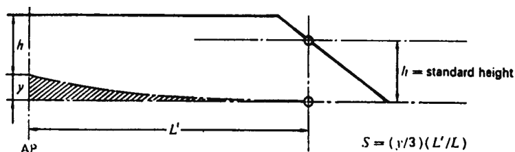
Figure 38.3 Shear credit S for excess height
