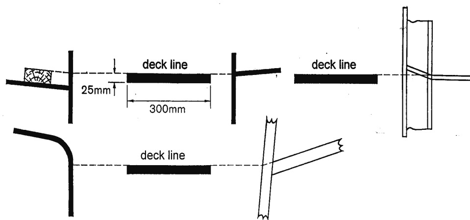
Figure 4.1 Deck line
